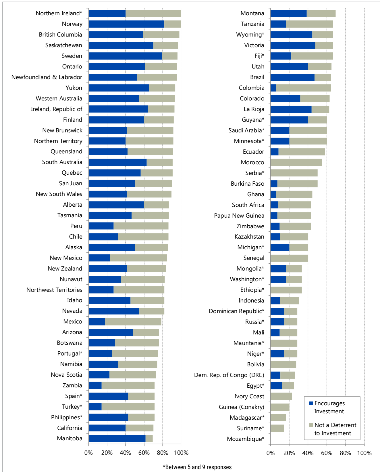
Figure 27: Geological Database
