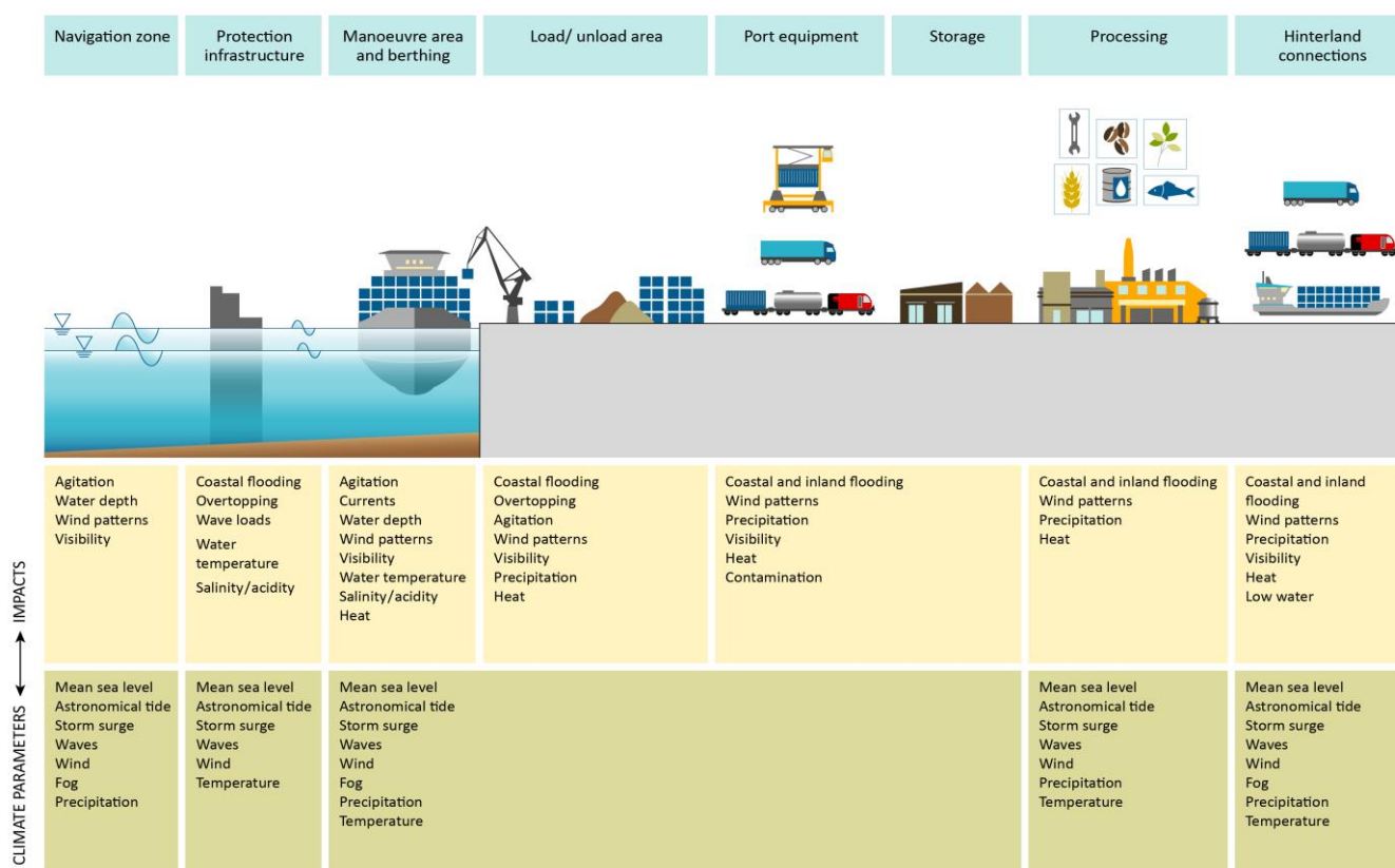
Figure 1: Interactions between climate parameters and processes and representative port assets and operations
