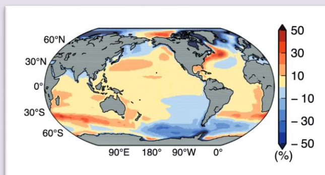
Box 10: Percentage of the deviation of the ensemble mean regional relative sea level change between 1986-2005 and 2081-2100 from the global mean value
