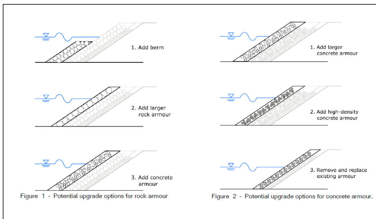
Figure 12: Retrofitting options for a breakwater or seawall
