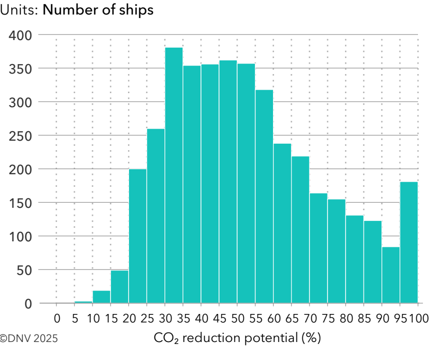
FIGURE 7-4 Number of containerships above 2 000 TEU (3 954 ships in total) with different annual CO 2 reduction potentials from onboard CO 2 capture, assuming given tank volumes and 100% capture rate
