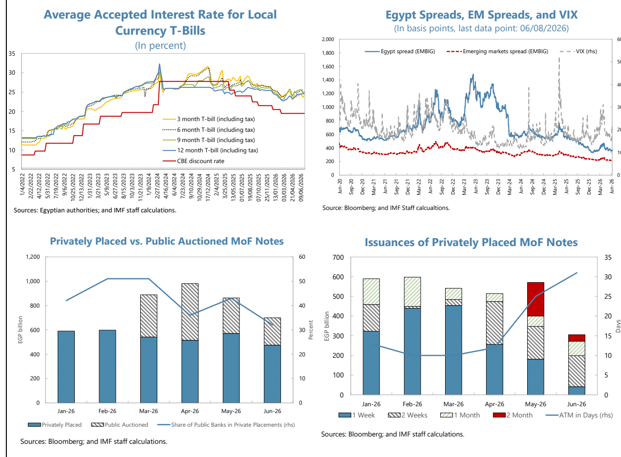
Figure 14. Egypt: Financing
